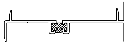
10940 Stack Mullion for 4 1/8" Window
